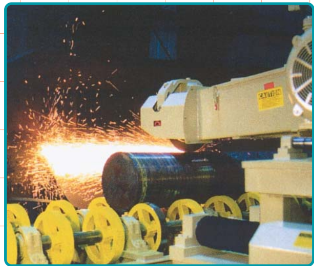
Rounds Rotator
