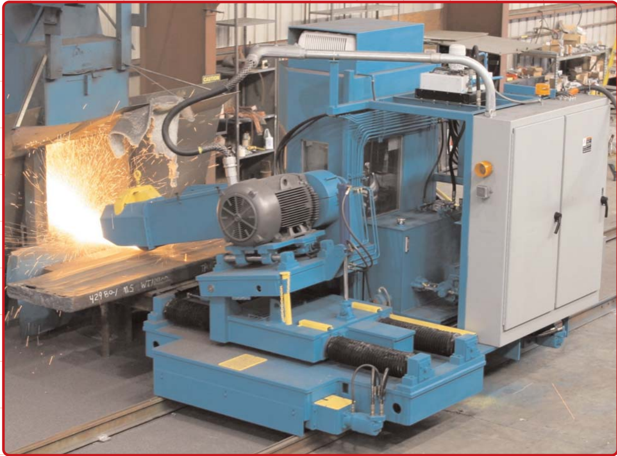
Model 6040T Traveling Grinder - 90°
